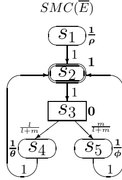
FIG. 2. The underlying SMC of \bar{E} for E = [(\{a\}, \rho) * ((\{b\}, \mathfrak{d}_k^1); (((\{c\}, \mathfrak{d}_l^0); (\{d\}, \theta)) \square ((\{e\}, \mathfrak{d}_m^0); (\{f\}, \phi)))) * \text{Stop}]
