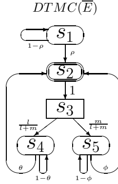
FIG. 3. The DTMC of \bar{E} for E = [(\{a\}, \rho) * ((\{b\}, \mathfrak{q}_k^1); (((\{c\}, \mathfrak{q}_l^0); (\{d\}, \theta)) [((\{e\}, \mathfrak{q}_m^0); (\{f\}, \phi))]) * \text{Stop}]
