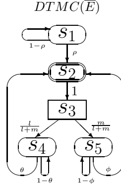
FIG. 3. The DTMC of \bar{E} for E = [(\{a\}, \rho) * ((\{b\}, \natural_k^1); (((\{c\}, \natural_l^0); (\{d\}, \theta)) [((\{e\}, \natural_m^0); (\{f\}, \phi)))) * \text{Stop}]
