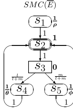
FIG. 2. The underlying SMC of \bar{E} for E = [(\{a\}, \rho) * ((\{b\}, \mathfrak{h}_k^1); ((\{c\}, \mathfrak{h}_l^0); (\{d\}, \theta)) \square ((\{e\}, \mathfrak{h}_m^0); (\{f\}, \phi)))] * \text{Stop}
