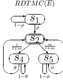
FIG. 4. The reduced DTMC of \bar{E} for E = [(\{a\}, \rho) * ((\{b\}, \eta_k^1); ((\{c\}, \eta_l^0); (\{d\}, \theta)) \parallel ((\{e\}, \eta_m^0); (\{f\}, \phi)))] * \text{Stop}
