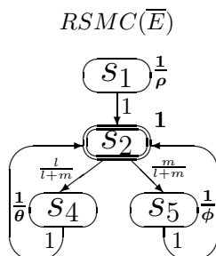
FIG. 5. The reduced SMC of \bar{E} for E = [(\{a\}, \rho) * ((\{b\}, \mathfrak{h}_k^1); ((\{c\}, \mathfrak{h}_l^0); (\{d\}, \theta)) \parallel ((\{e\}, \mathfrak{h}_m^0); (\{f\}, \phi)))] * \text{Stop}
