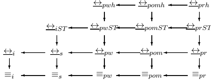
Figure 1. Correlation of the equivalences
