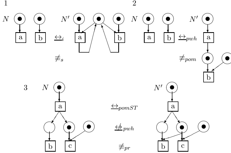
Figure 6. Examples of strictly labelled nets
