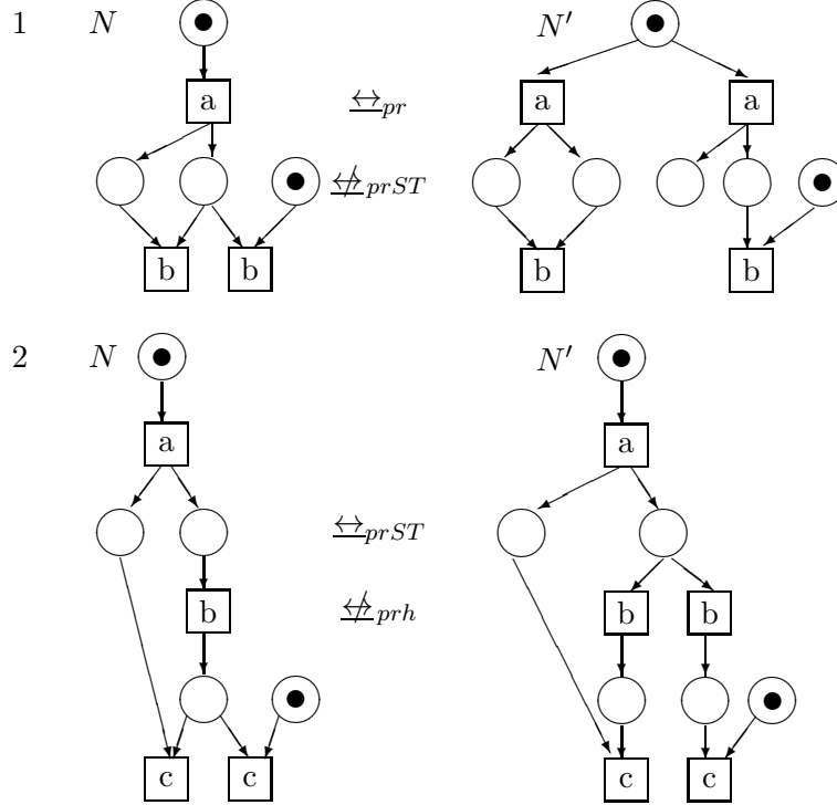
Figure 5. Examples of sequential nets
